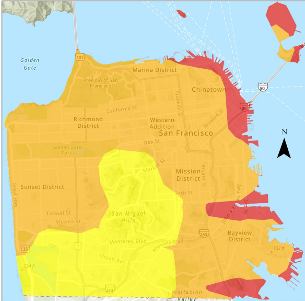
FIGURE 4-8 PREDICTED GROUND SHAKING INTENSITY: 7.0 HAYWARD FAULT SCENARIO
