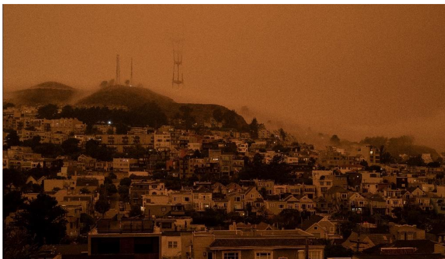
Wildfire Smoke Causing "Orange Sky Day" in 2020
