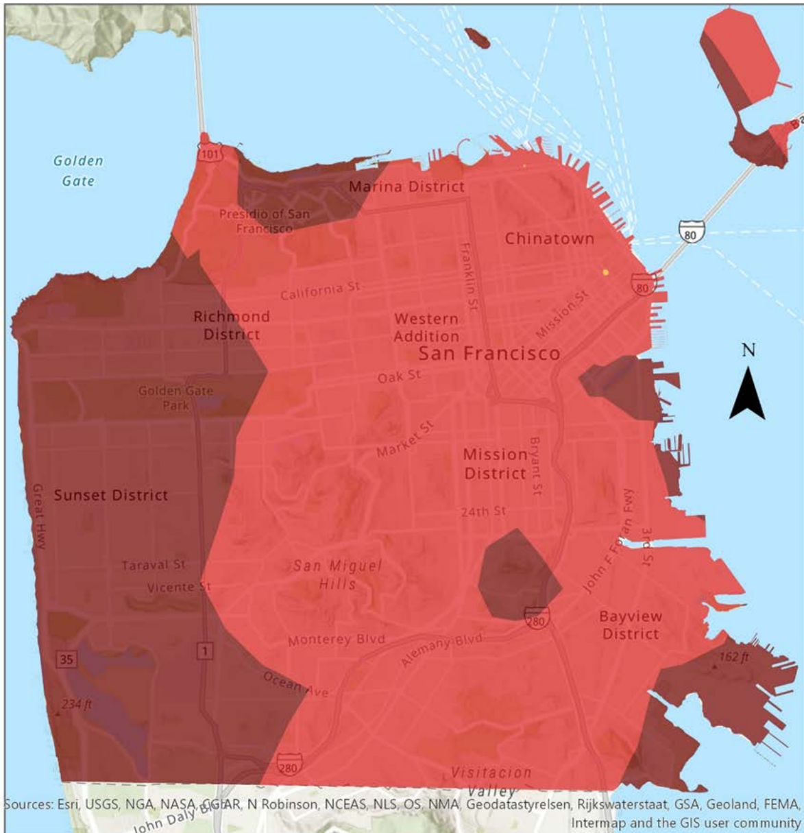
FIGURE 4-3 PREDICTED GROUND SHAKING INTENSITY: 7.8 SAN ANDREAS FAULT SCENARIO
