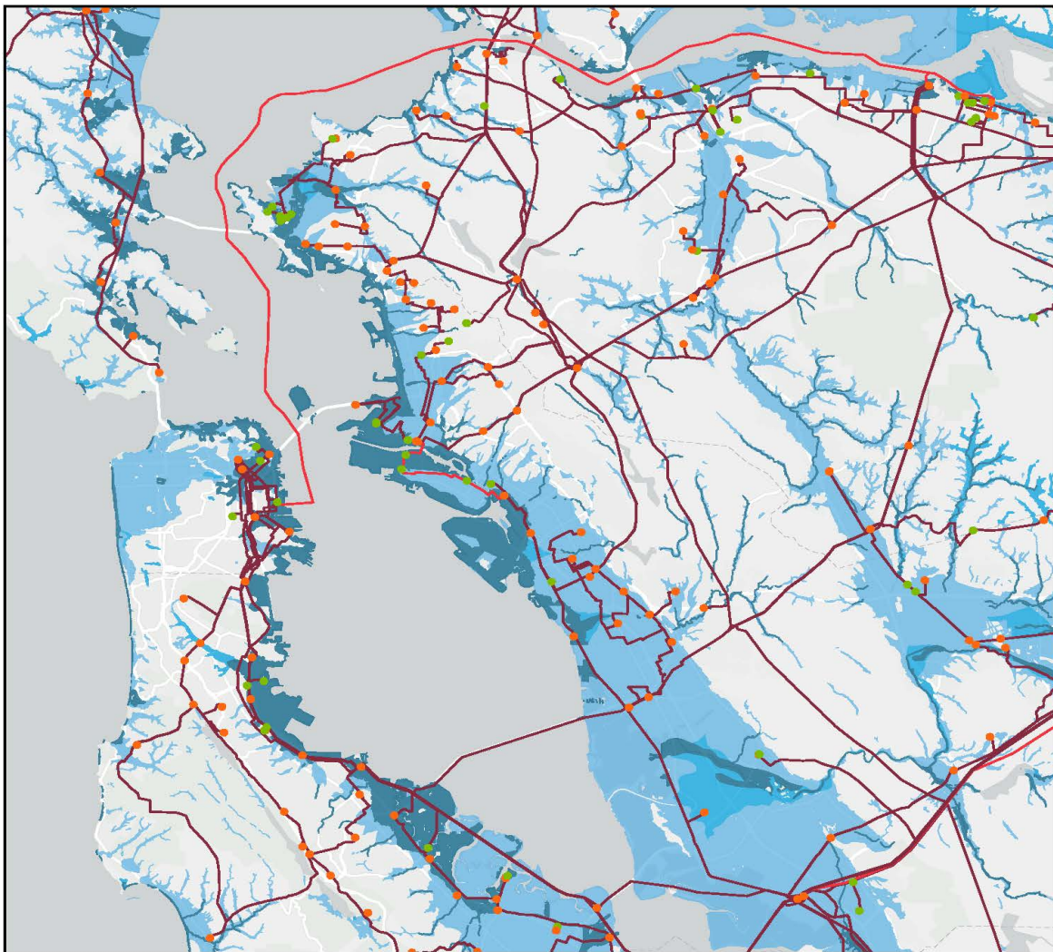
FIGURE 7: ELECTRIC POWER SYSTEM MAP
