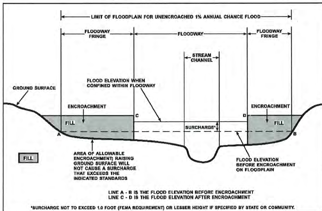
Figure 4: Floodway Schematic
